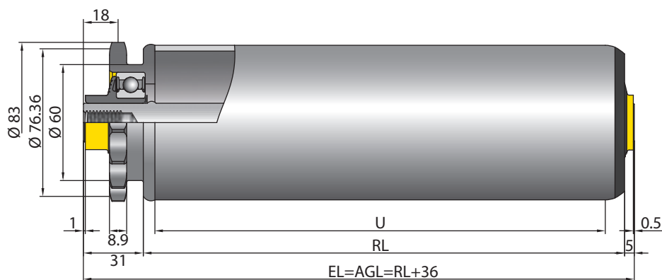
Welded 5/8" steel double sprocket head with 15 teeth
