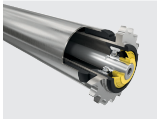
Double friction conveyor roller Series 3880 | page 136
