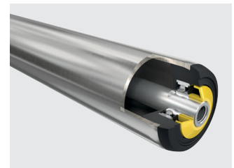
Universal conveyor roller Series 1700 heavy | page 72
