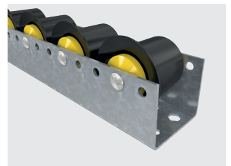
Roller track Series BU50 | page 184
