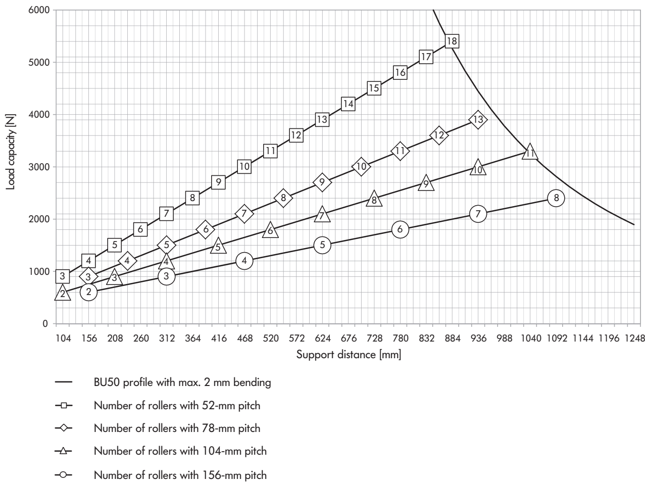
Fig.: Roller track with polymer rollers
