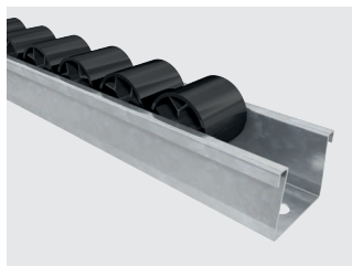
Wheel track Floway Series | page 176
