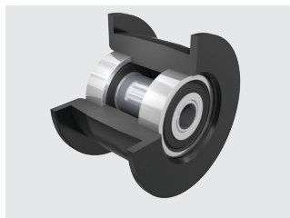
Pressure roller Series 2600 | page 160
