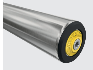
Heavy-duty universal conveyor roller Series 1450 | page 42
