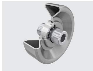
Steel conveyor wheel Series 2200 | page 154
