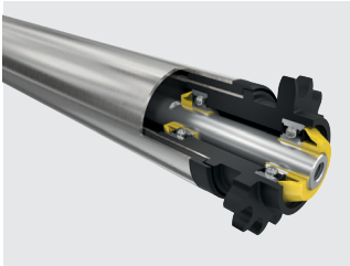
Double friction conveyor roller Series 3870 | page 130
