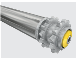
Fixed drive conveyor roller Series 3500 heavy | page 102
